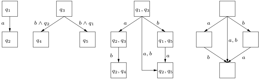
Fig. 9. Two interacting systems and their composition (the transition label a, b indicates that a and b occur simultaneously); a confluent automaton
