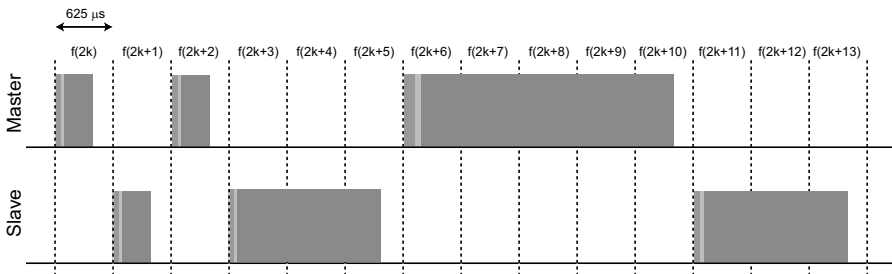
Fig. 3. The TDD scheme used in Bluetooth
