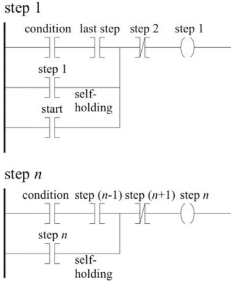
Fig. 9. Sequencing execution described in LD notation
