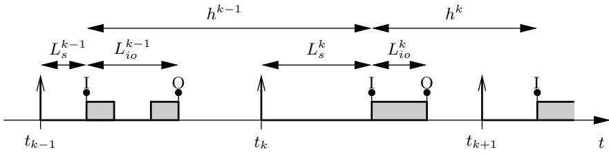
Fig. 1. Controller timing
