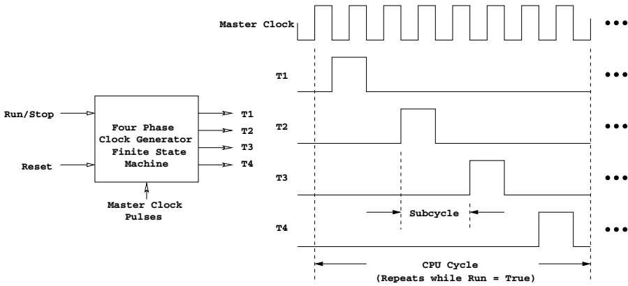
Fig. 9. Four-phase clock
