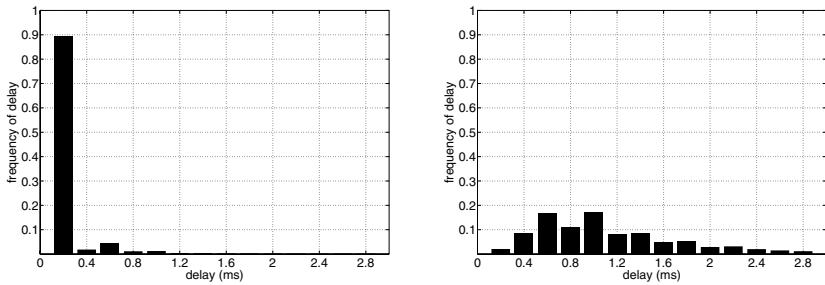
(a) UDP delays, 3Mbit/sec cross-traffic (b) UDP delays, 22Mbit/sec cross-traffic
