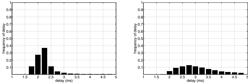
(c) OPC delays, 3Mbit/sec cross-traffic (d) OPC delays, 22Mbit/sec cross-traffic
