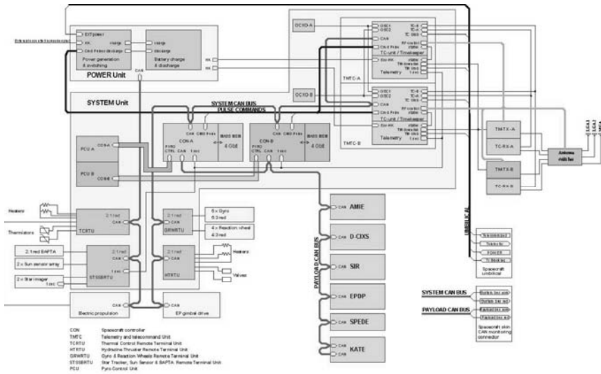
Fig. 10. Part of the distributed control architecture for the SMART-1 spacecraft. The system has two CAN buses: one for the control of the spacecraft and one for the payload. The spacecraft controllers are redundant and denoted CON-A and CON-B in the middle of the block diagram. (Courtesy of the Swedish Space Corporation.)
