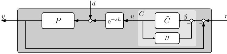
Fig. 5. Dead-time compensator
