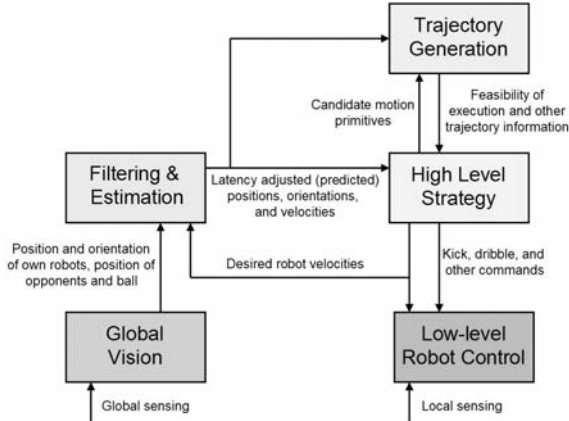
Fig. 4. Functional architecture
