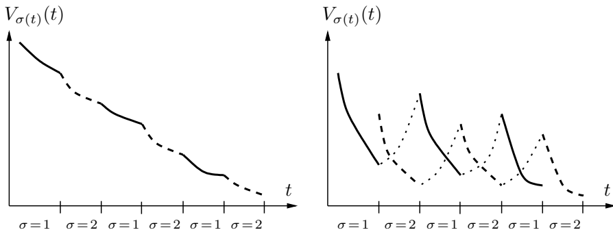
Fig. 3. Two Lyapunov functions (solid graphs correspond to V_1 , dashed graphs correspond to V_2 ): (left) continuous V_\sigma , (right) discontinuous V_\sigma
